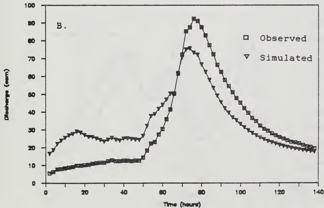
Figure 29. (A) Hyetograph, and (B) simulated and observed hydrographs for a "simple" rainfall event on Flynn Creek, Oregon Coast Range (March 6-12, 1966). The API method tends to over-estimate rising limb runoff and under-estimate falling limb runoff.
